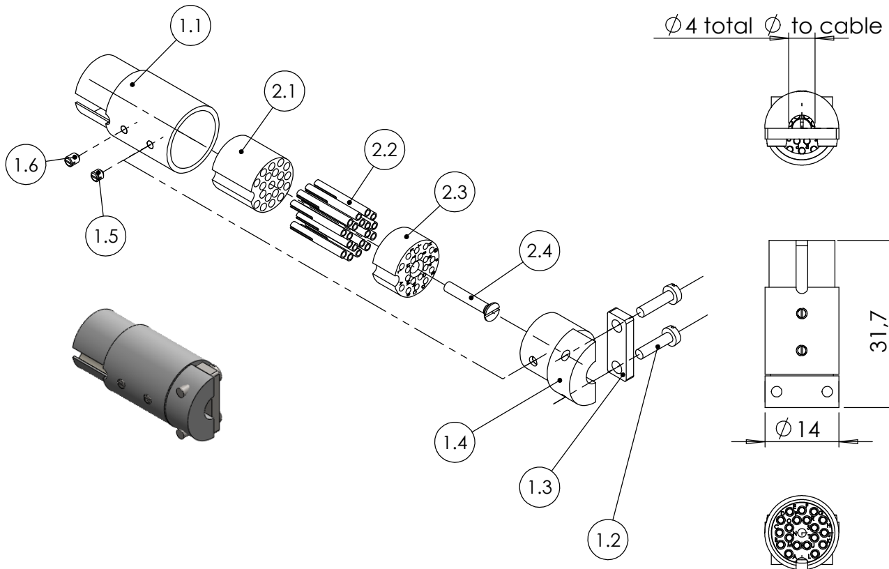
view feedthrough
